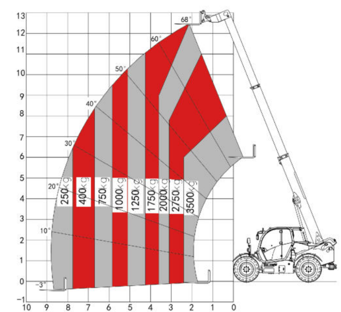
35THCJ13-Q/Q1/CU 载荷曲线图 Lifting diagram
